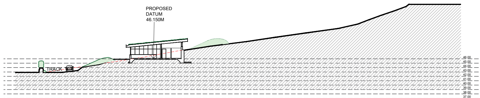
PROPOSED SITE SECTION A-A 1:500
