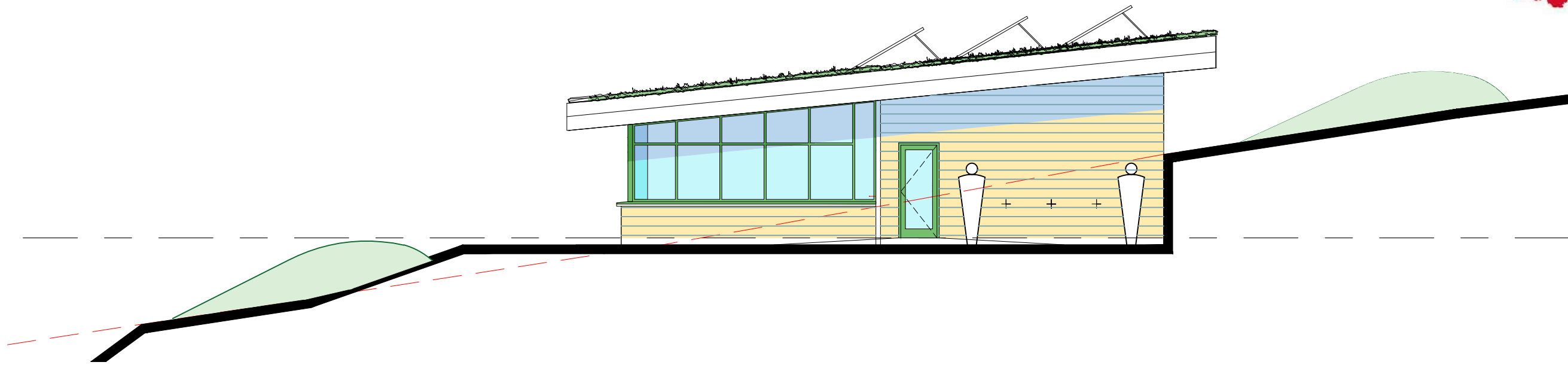
PROPOSED EAST ELEVATION 1:100
