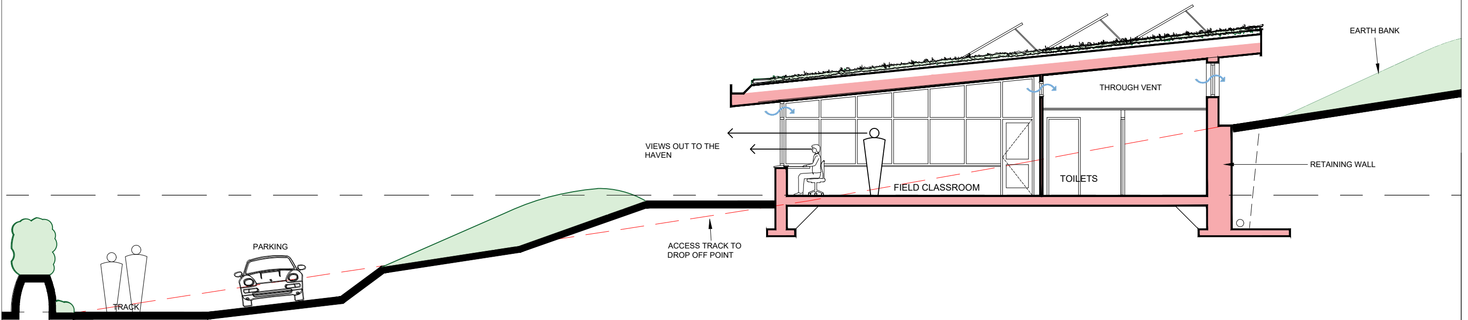
PROPOSED SECTION 1:100
